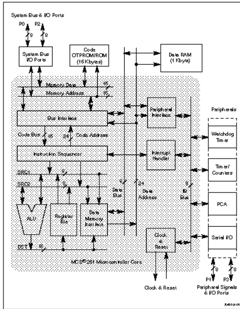
Figure 1. 8XC251SB Functional Block Diagram
