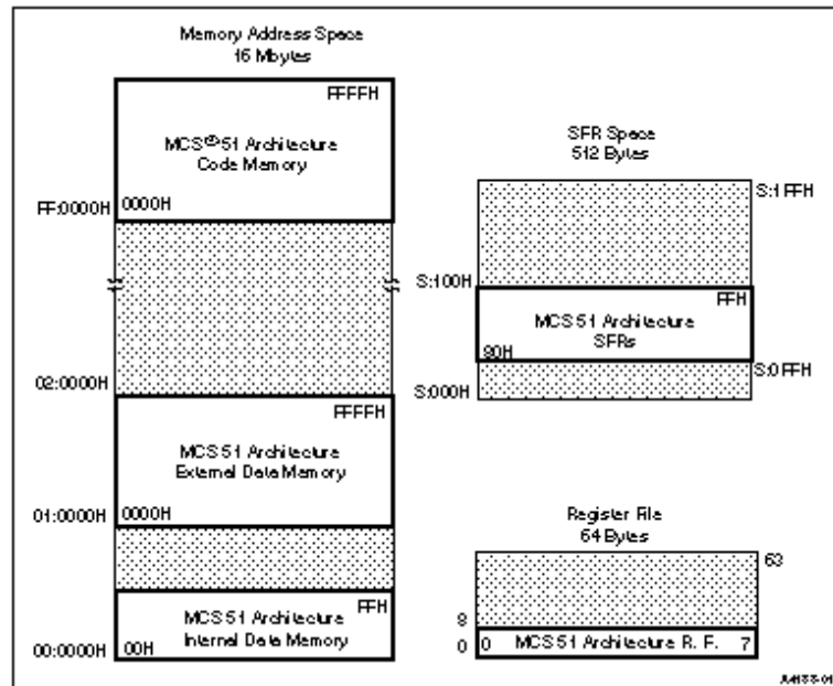
Figure 2. MCS ® 51 Memory Mapping in 8XC251SB
