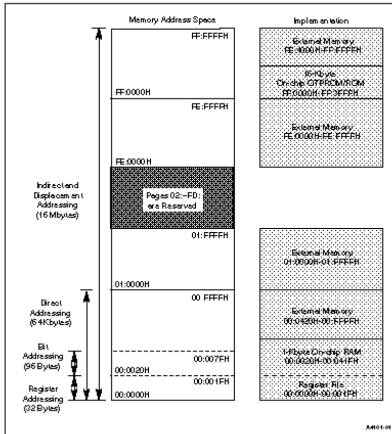
Figure 3. 8XC251SB Memory Mapping
