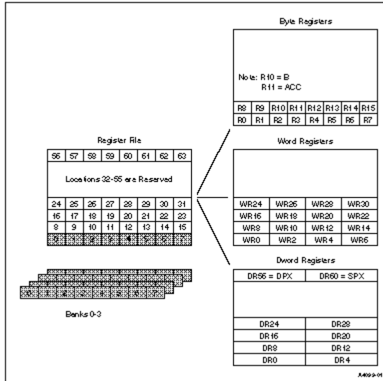
Figure 4. 8XC251SB Register File
