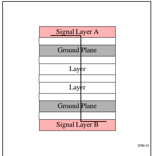
Figure 10. Layer Switch with Multiple Reference Planes (same type)
