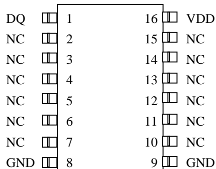
DS2434 16-Pin SSOP See Mech. Drawings Section
