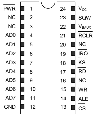
DS1687 24-Pin Encapsulated
