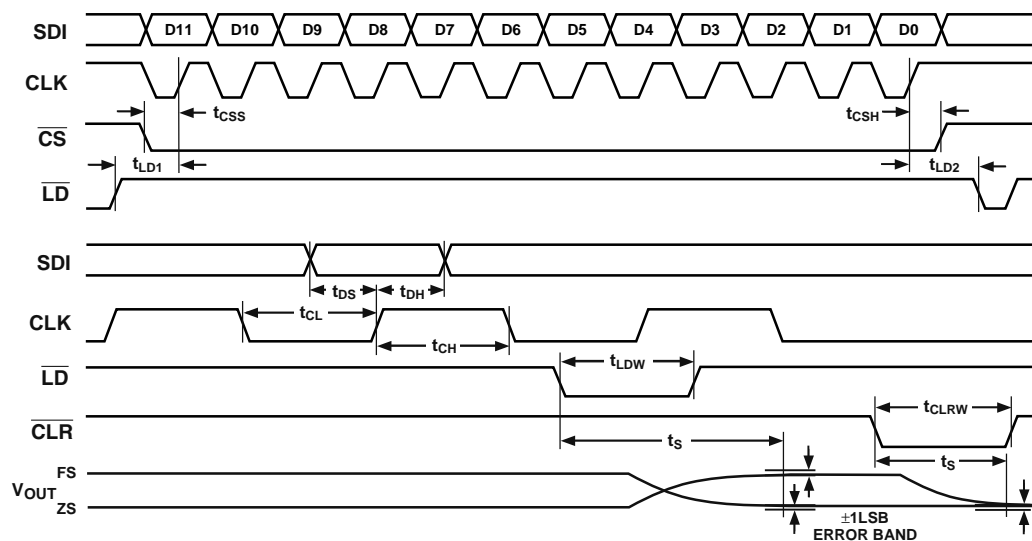
Figure 3. Timing Diagram
