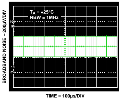
Figure 5. Broadband Noise
