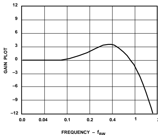
Figure 4. Gain Plot
