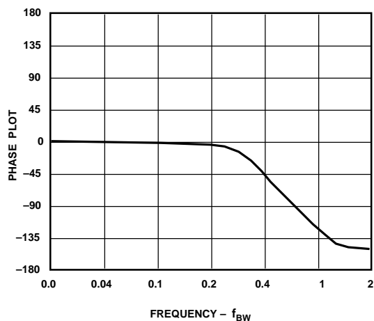
Figure 5. Phase Plot
