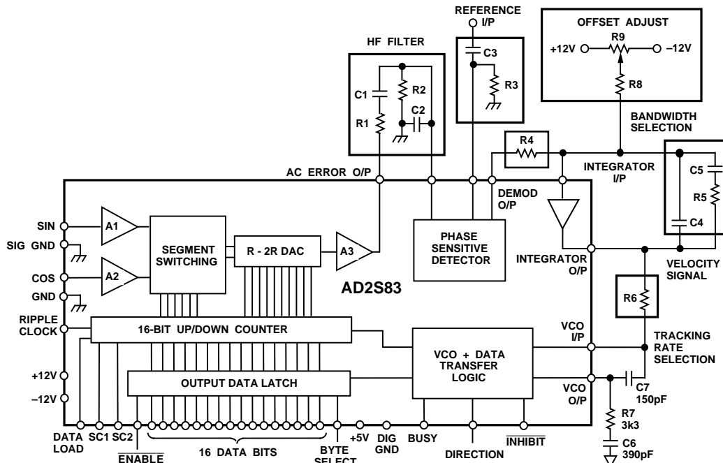
Figure 1. Connection Diagram
