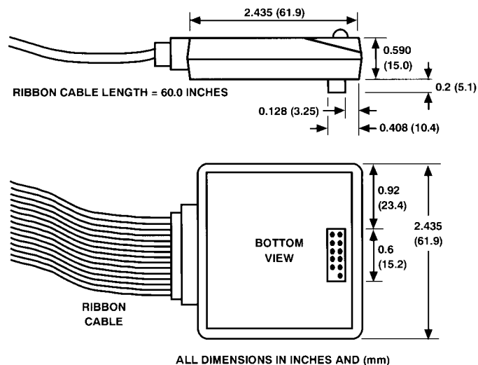
Figure 21. EZ-ICE Probe
