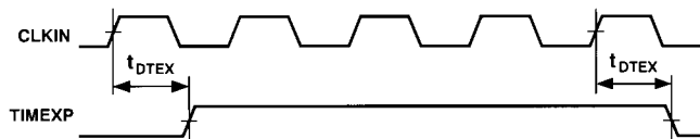
Figure 6. TIMEXP
