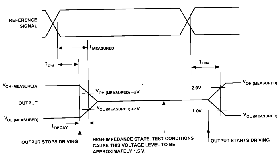
Figure 13. Output Enable/Disable
