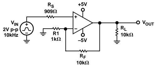
Figure 34. Overload Recovery Time Test Circuit
