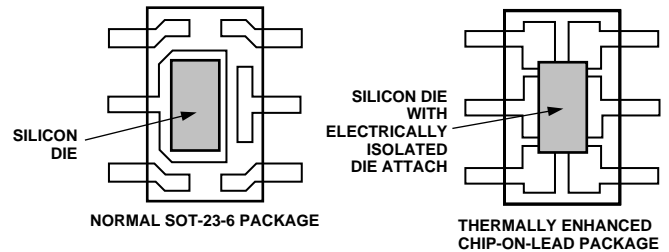
Figure 22. Chip-on-Lead Package
