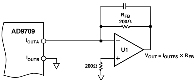
Figure 37. Unipolar Buffered Voltage Output
