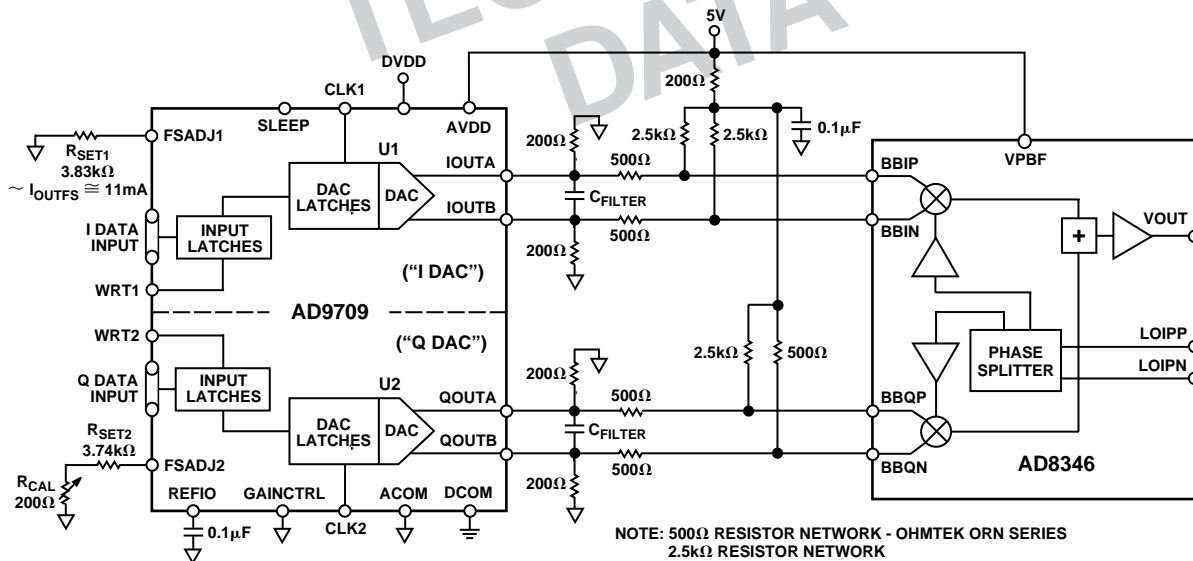
Figure 41. Baseband QAM Implementation Using an AD9709 and AD8346
