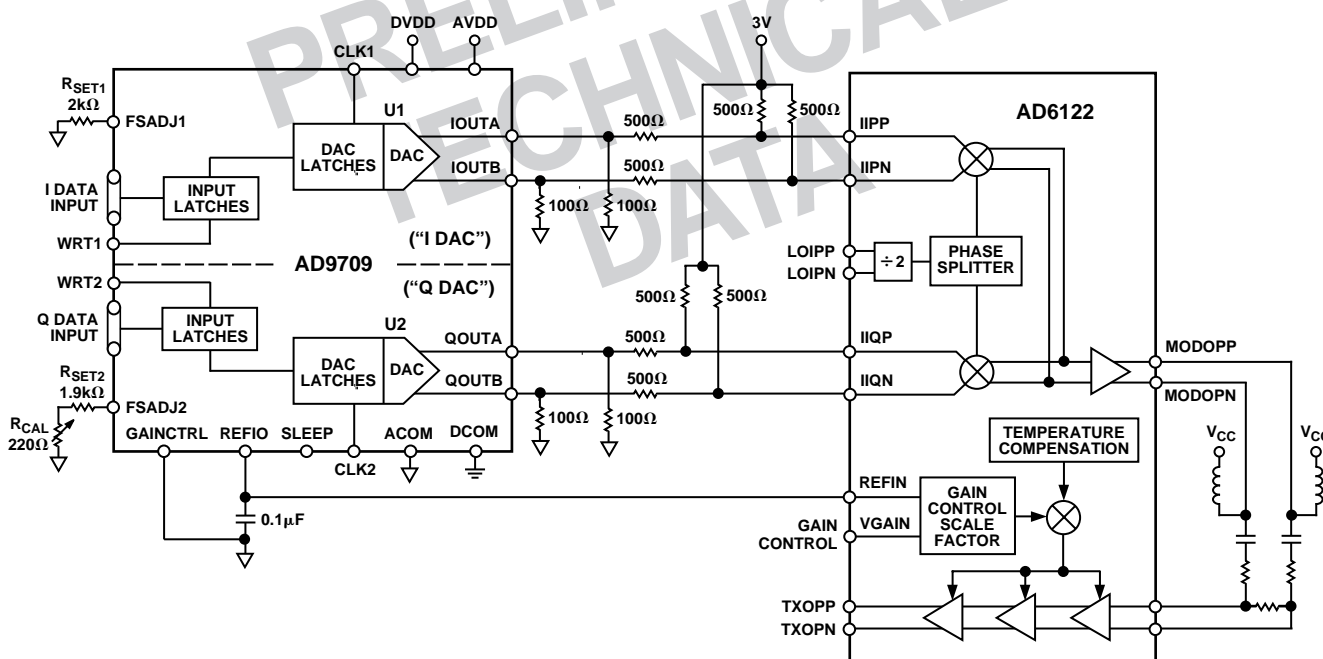
Figure 43. CDMA Transmit Application Using AD9709 and AD6122
