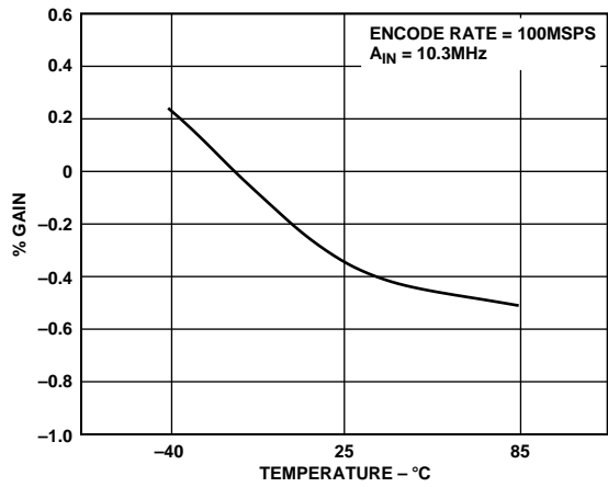
Figure 15. ADC Gain vs. Temperature (with External +1.25 V Reference)
