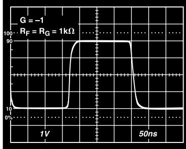
Figure 22. Driver 4 V Step Response, G = -1
