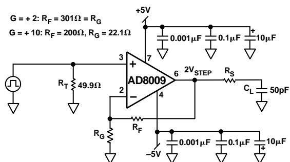
Figure 39. AD8009 Capacitive Load Drive Circuit
