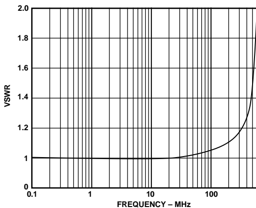
Figure 23. Input VSWR; G = +10
