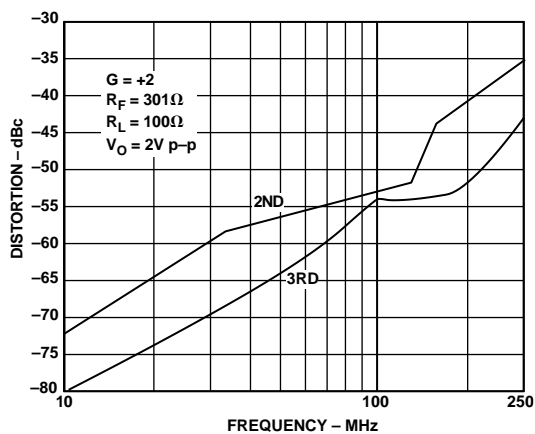
Figure 10. Distortion vs. Frequency; G = +2
