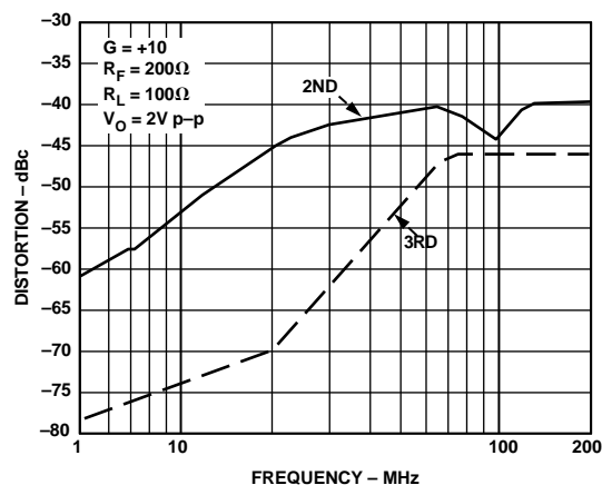
Figure 13. Distortion vs. Frequency; G = +10
