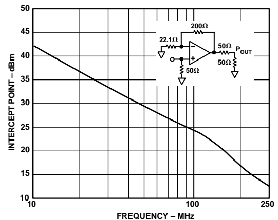
Figure 15. Two Tone, 3rd Order IMD Intercept vs. Frequency; G = +10
