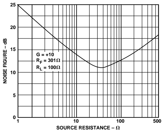
Figure 22. Noise Figure
