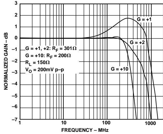
Figure 4. Frequency Response; G = +1, +2, +10
