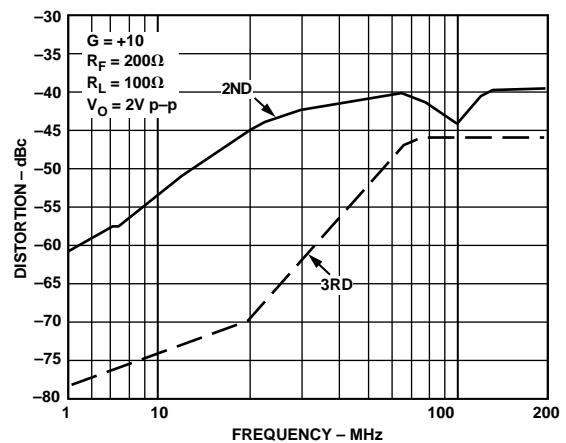
Figure 2. Distortion vs. Frequency; G = +10
