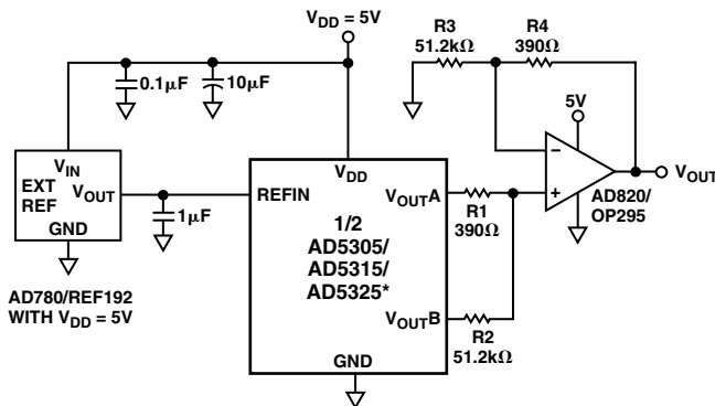
Figure 38. Coarse/Fine Adjustment
