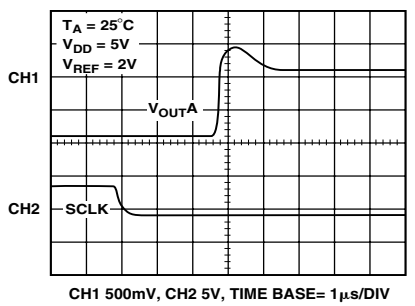
Figure 21. Exiting Power-Down to Midscale
