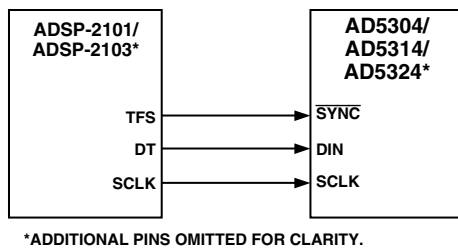
Figure 33. AD5304/AD5314/AD5324 to ADSP-2101/ADSP-2103 Interface
