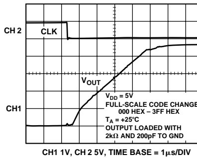
Figure 15. Full-Scale Settling Time
