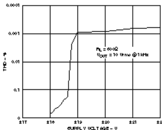
Figure 5. THD + Noise vs. Supply Voltage
