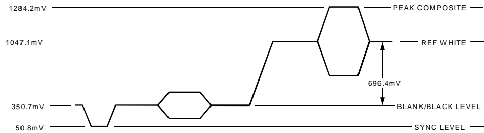
Figure 112. PAL Composite Video Levels
