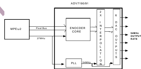
Figure xx PLL and 4xOversampling block diagram
