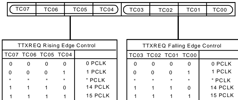
Figure 69 . Teletext Request Control Register
