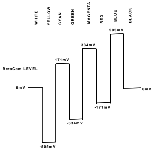
Figure 130. NTSC 100% Color Bars No Pedestal U Levels
