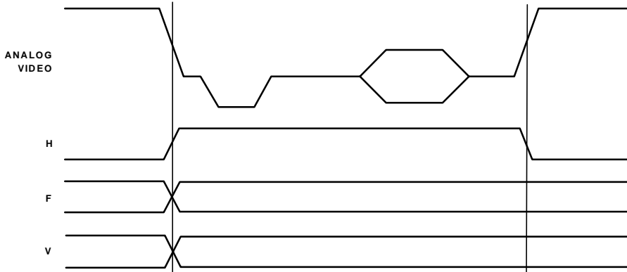
Figure 36. Timing Mode 0 Data Transitions (Master Mode)
