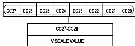
Figure 74. Color Control Registers
