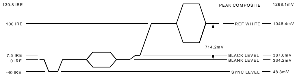
Figure 104. NTSC Composite Video Levels
