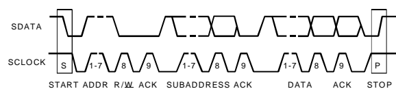
Figure 47. Bus Data Transfer
