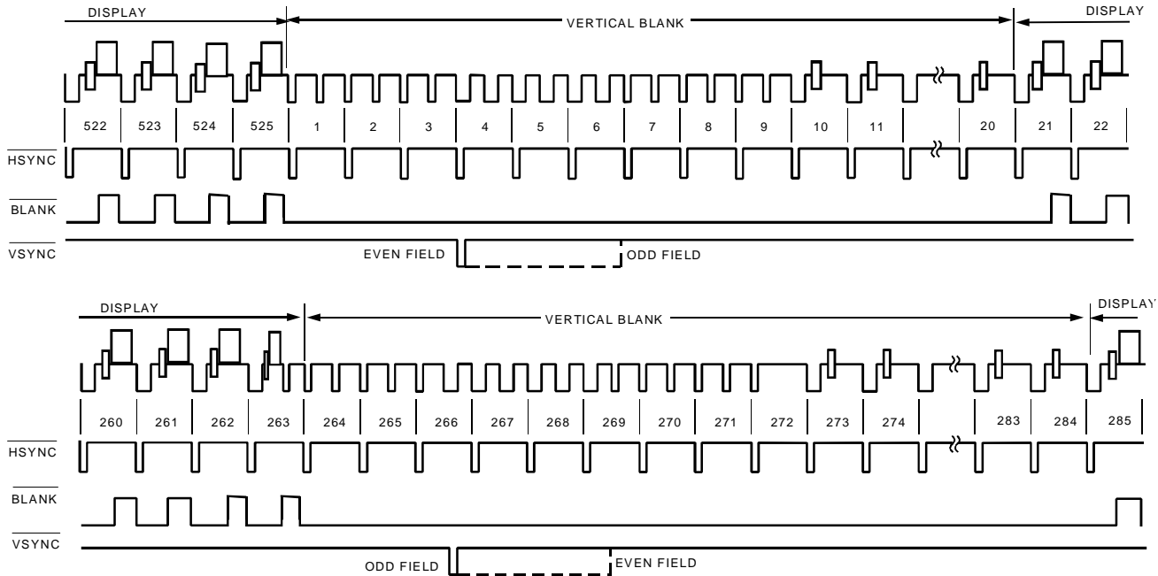
Figure 40 Timing Mode 2 (NTSC)
