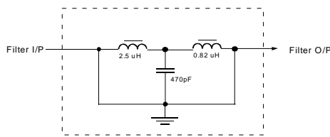
Figure 97. Output Filter for 2xOversampling Mode
