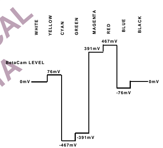
Figure 133. NTSC 100% Color Bars with Pedestal V Levels
