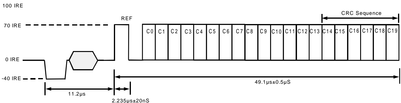
Figure 93. CGMS Waveform diagram
