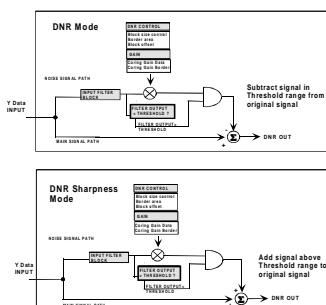
Figure xx Block diagram for DNR Mode and DNR Sharpness Mode
