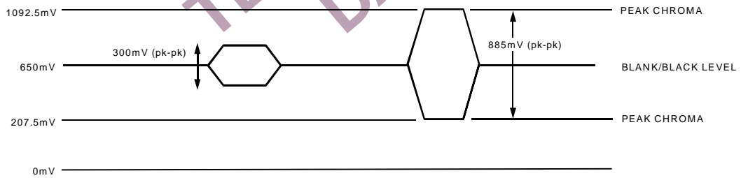
Figure 114. PAL Chroma Video Levels
