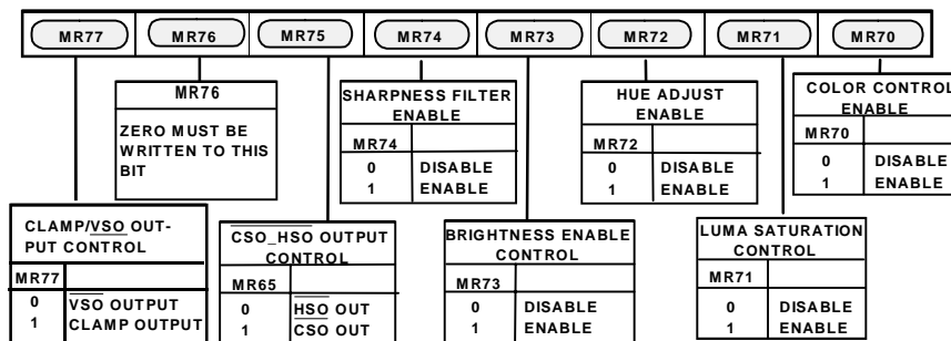
Figure 57. Mode Register 7 (MR7)
