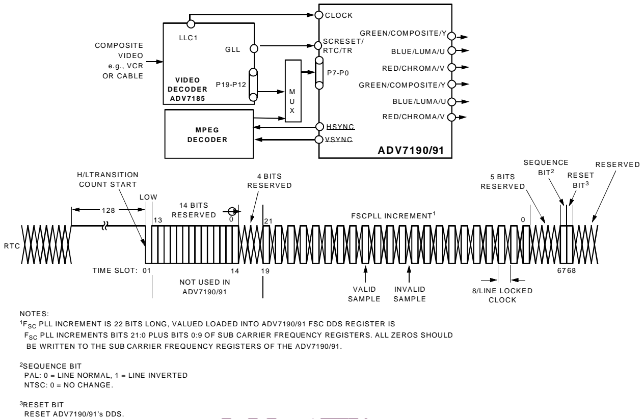
Figure 32. RTC Timing and Connections
