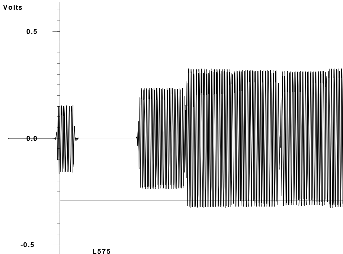
Figure 138 100/75% PAL Color Bars Chrominance
