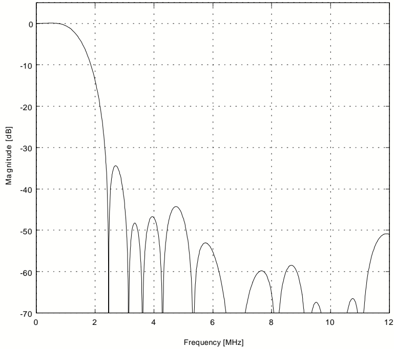
PRELIMINARY TECHNICAL DATA Figure 20 Chroma 1.3MHz Low Pass Filter (4xOversampling)
