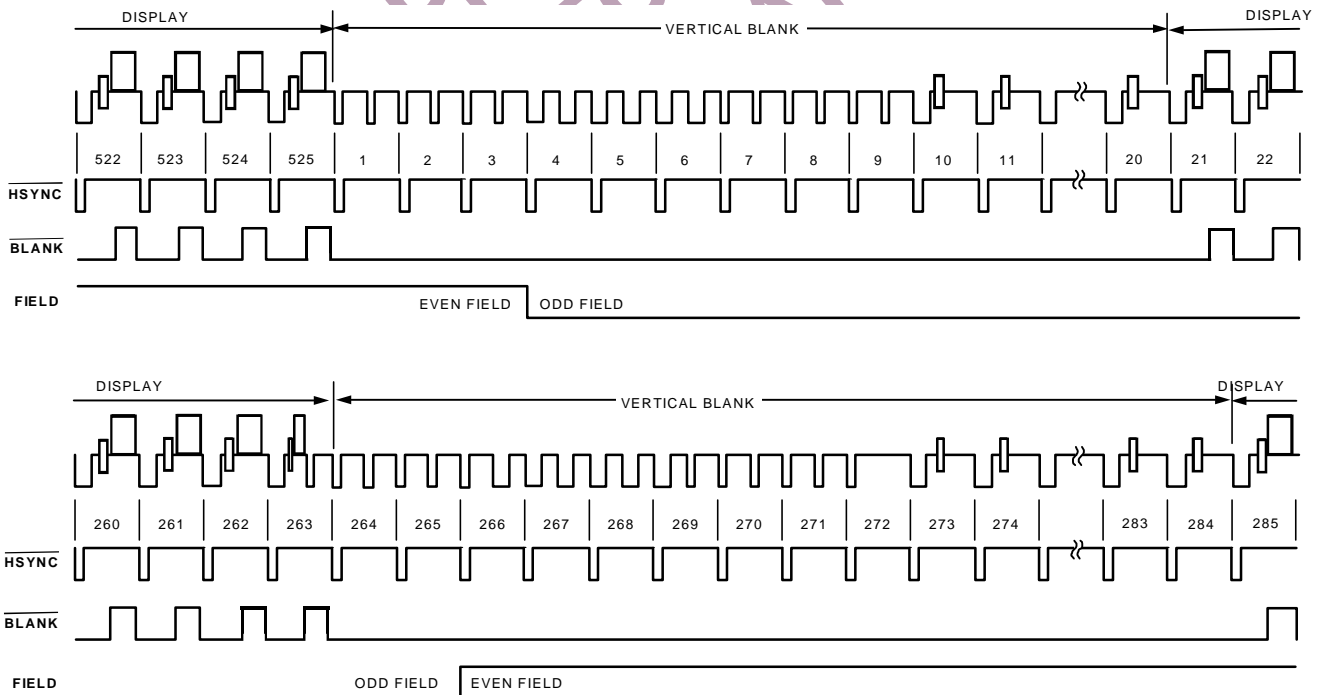
Figure 37. Timing Mode 1 (NTSC)
