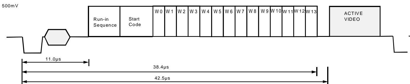
Figure 94. WSS Waveform diagram
