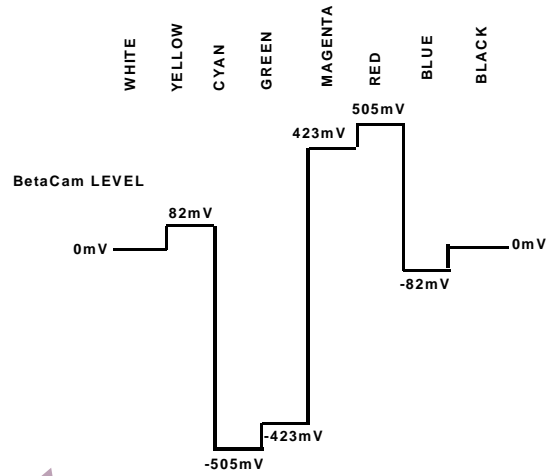
Figure 131. NTSC 100% Color Bars No Pedestal V Levels
