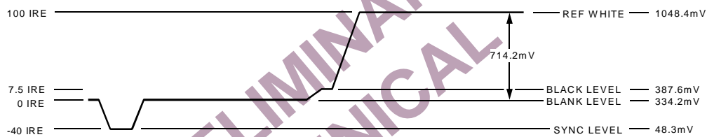
Figure 105. NTSC Luma Video Levels
