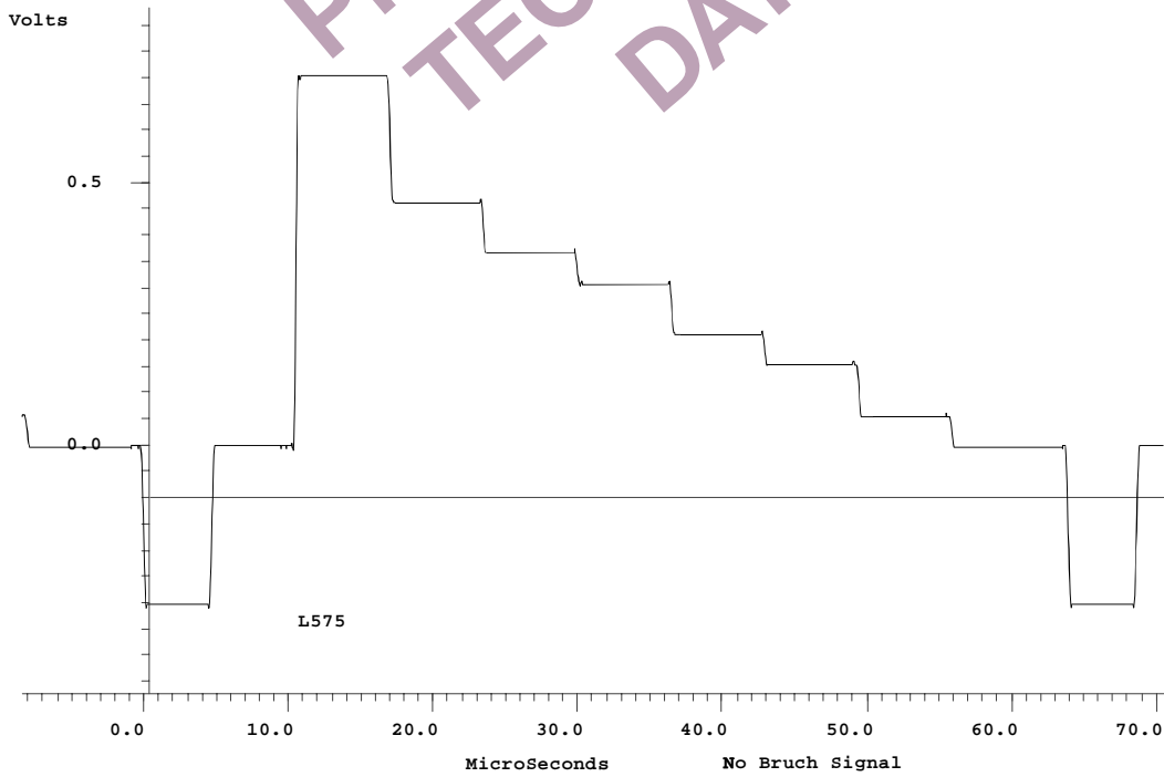
Figure 136. 100/75% PAL Color Bars
