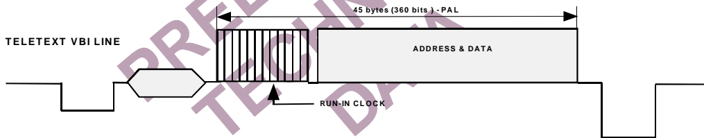
Figure 95. Teletext VBI Line
