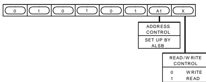
Fig 46. ADV7190/91 Slave Address
