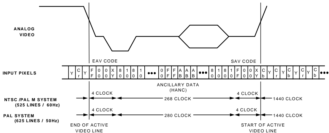
Figure 33. Timing Mode 0 (Slave Mode)
