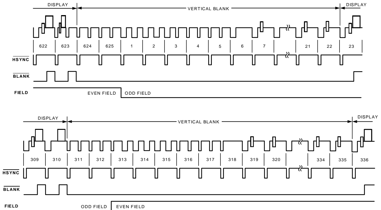
Figure 38 Timing Mode 1 (PAL)
