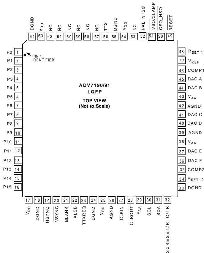
Figure 4. Pin Configuration ADV7190/91
