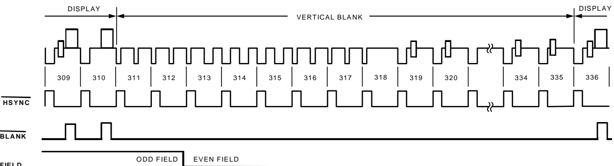
Figure 45. Timing Mode 3 (PAL)
