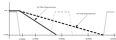
Figure xx. Output Filter Requirements in 2x- and 4xOversampling Mode
