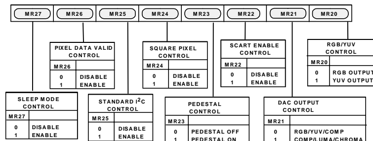
Figure 52. Mode Register 2 (MR2)
