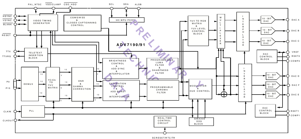
Figure 5 Detailed Block Diagram ADV7190/91
