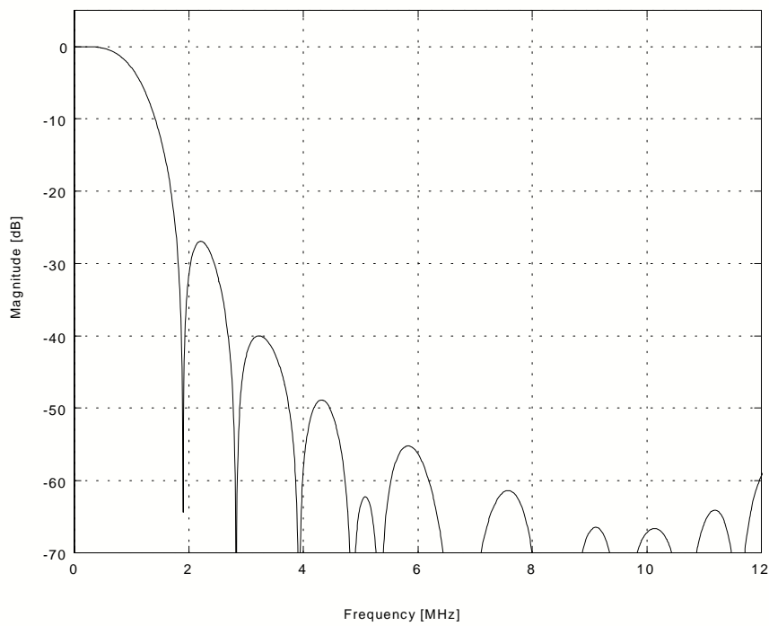
Figure 19 Chroma 1.0MHz Low Pass Filter (4xOversampling)
