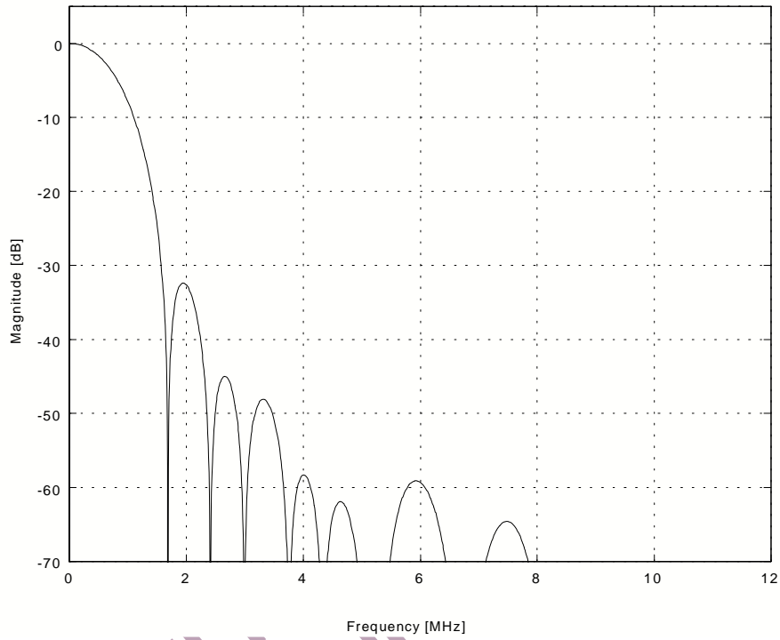
Figure 18 Chroma 0.65MHz Low Pass Filter (4xOversampling)
