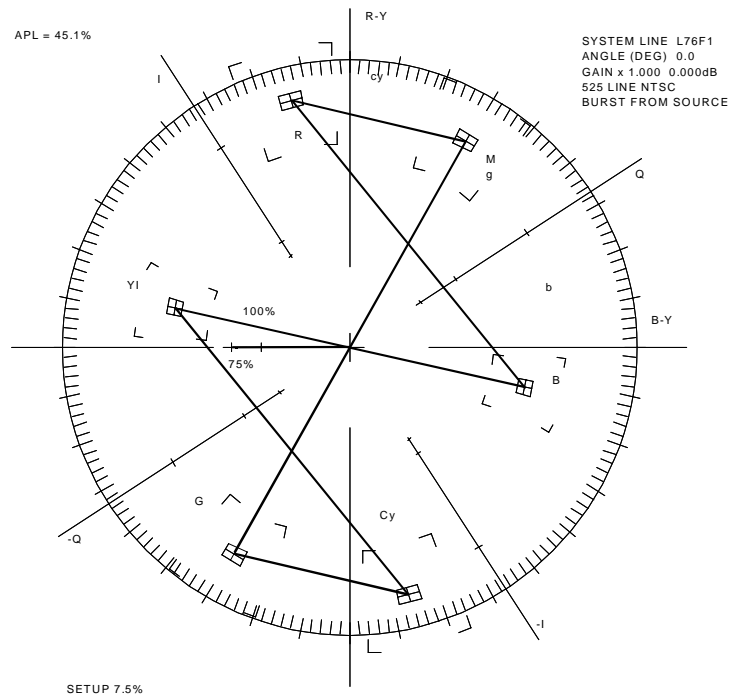
Figure 143. NTSC Vector Plot
