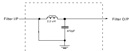
Figure 98. Output Filter for 4xOversampling Mode
