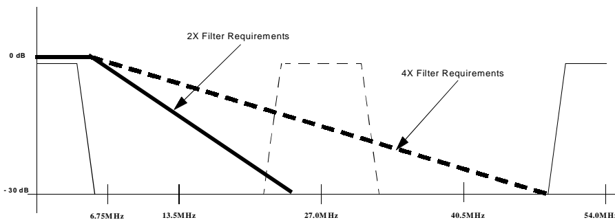
Figure 99. Output Filter Plot for 2xOversampling filter
