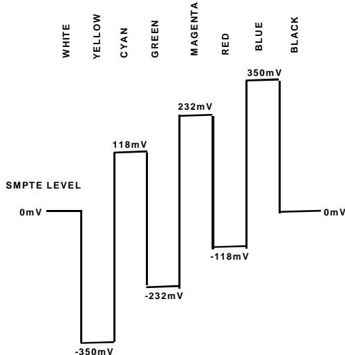
Figure 136. PAL 100% Color Bars U Levels
