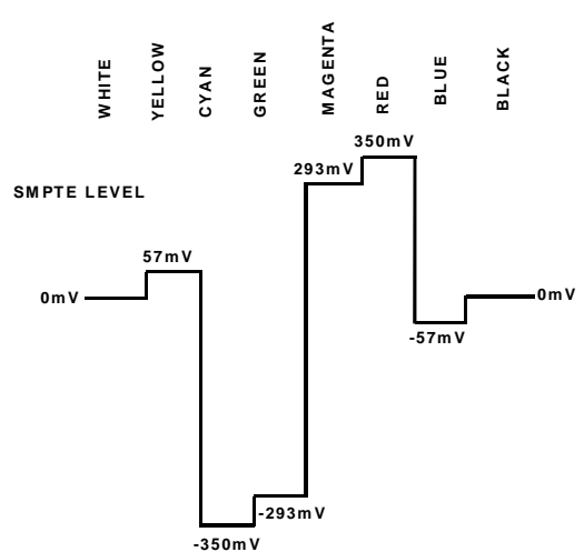
Figure 135-. PAL 100% Color Bars V Levels
