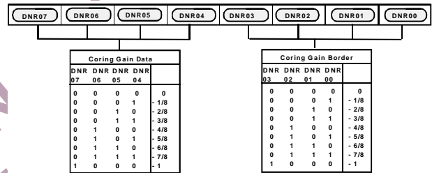
Figure 81. DNR Register 0 in DNR Mode
