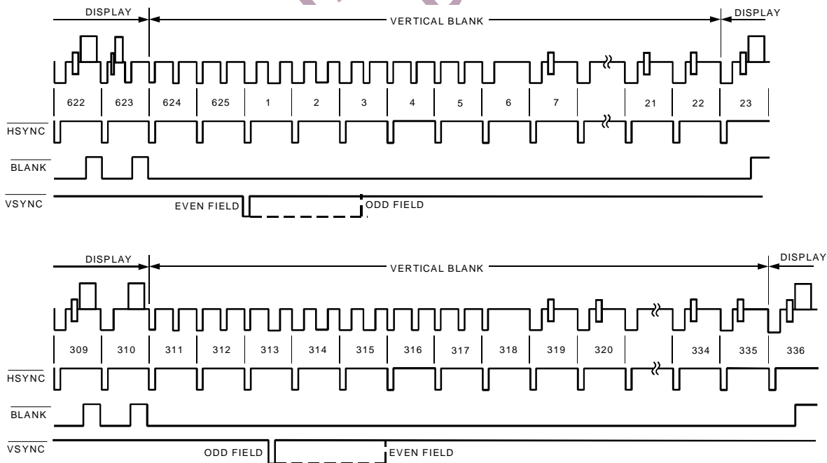
Figure 41. Timing Mode 2 (PAL)
