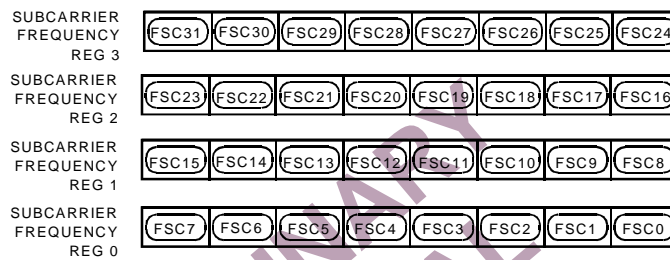
Figure 63. Sub Carrier Frequency Registers
