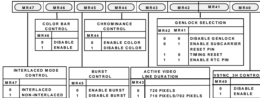
Figure 54. Mode Register 4 (MR4)
