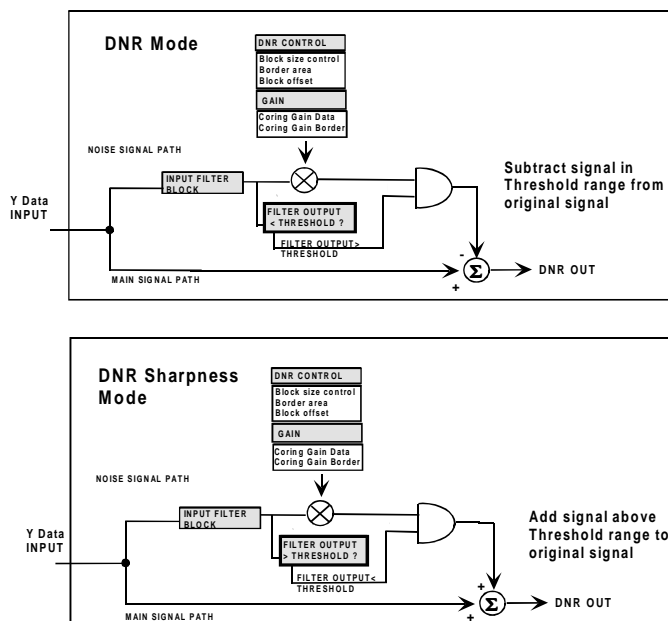
Figure 85 Block diagram for DNR Mode and DNR Sharpness Mode
