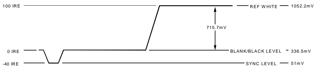
Figure 111. NTSC RGB Video Levels
