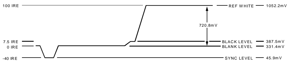
Figure 107. NTSC RGB Video Levels
