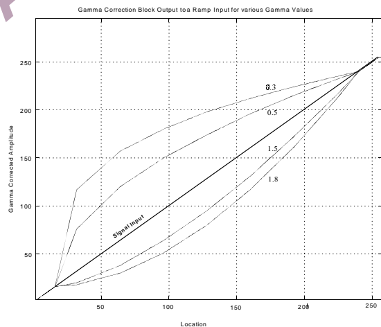
Figure 89 Signal Input (Ramp) and selectable Gamma Output curves
