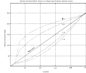
Figure xx Signal Input (Ramp) and selectable Gamma Output curves
