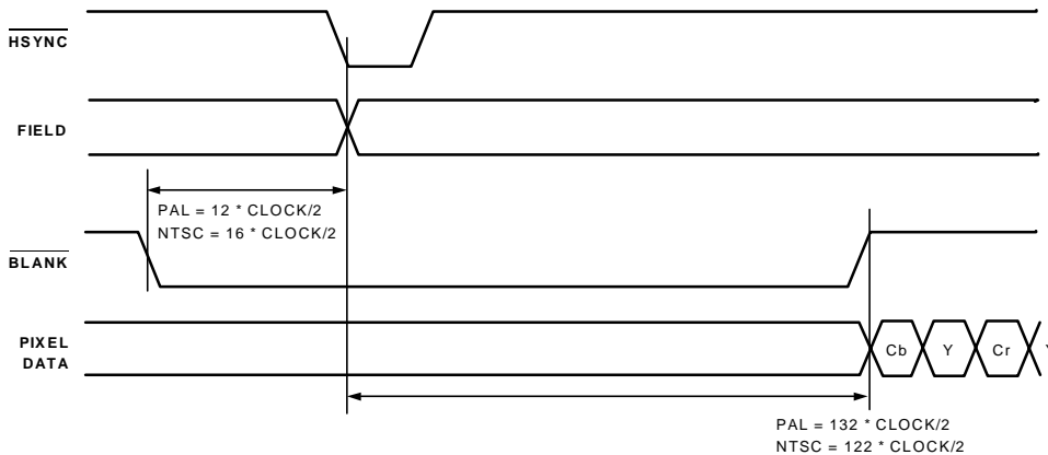
Figure 39. Timing Mode 1 Odd/Even Field Transitions Master/Slave
