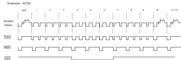
Figure 28 CSO, HSO, VSO timing diagram
