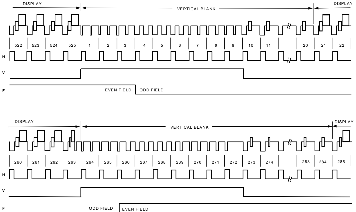
Figure 34. Timing Mode 0 (NTSC Master Mode)
