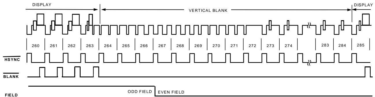
Figure 44. Timing Mode 3 (NTSC)
