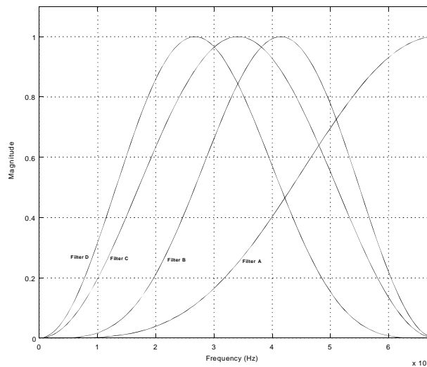
Figure 84. Filter Response of filters selectable
