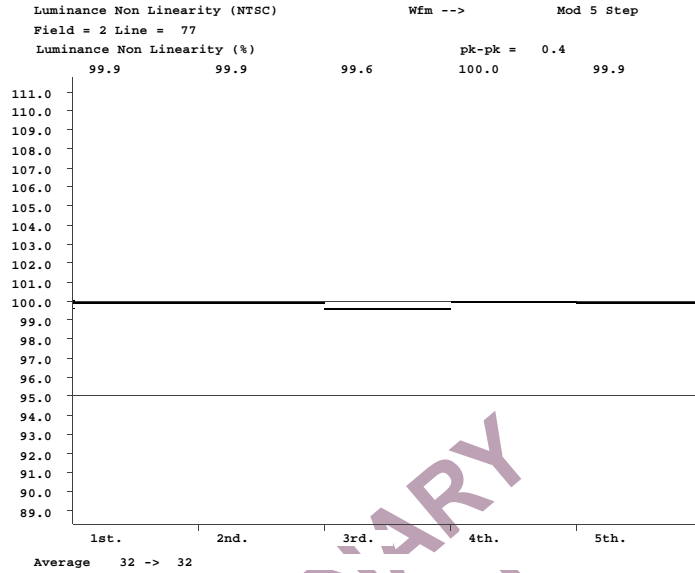
Figure 120. NTSC Luminance Non-Linearity
