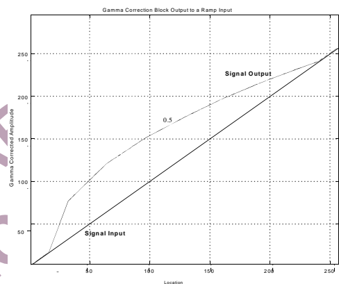
Figure 88 Signal Input (Ramp) and Signal Output for Gamma 0.5
