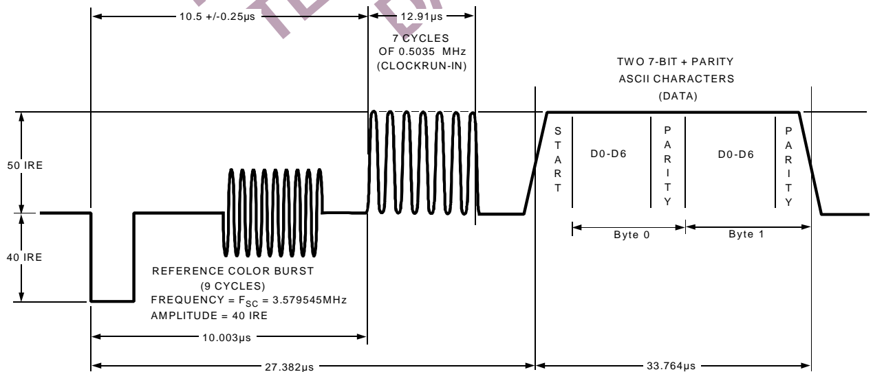
Figure 92. Closed Captioning Waveform (NTSC)
