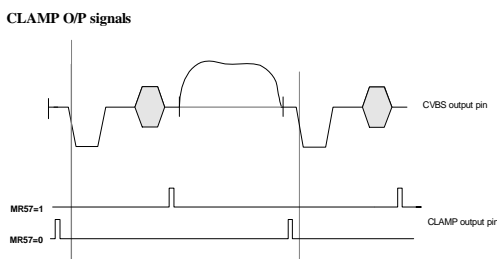
Figure 27 Clamp output timing
