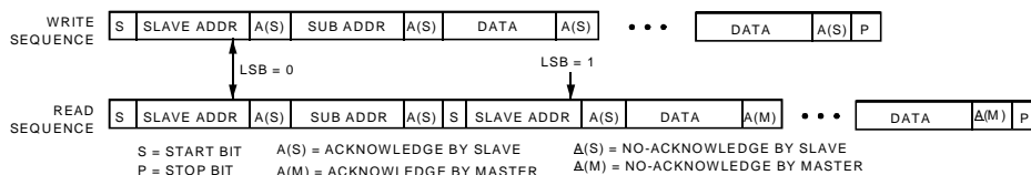
Figure 48 Write and Read Sequences
