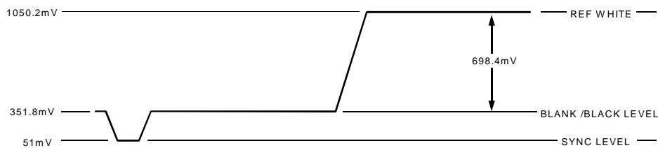
Figure 115. PAL RGB Video Levels
