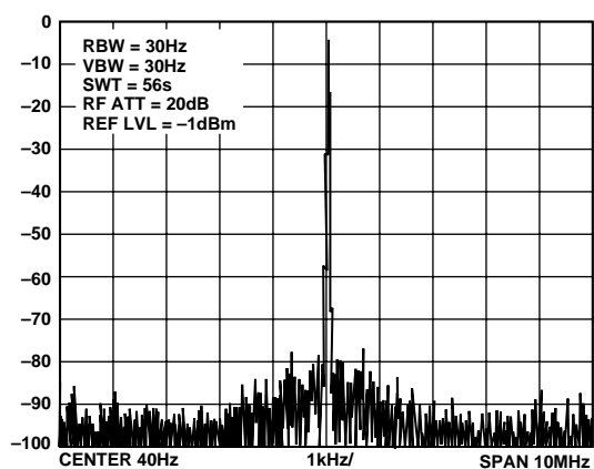
Figure 13. 6\times REFCLK Enabled
