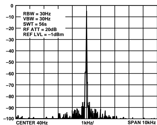
Figure 14. 6\times REFCLK Disabled
