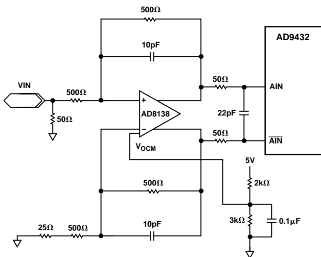
Figure 26. AD8138/AD9432 Schematic
