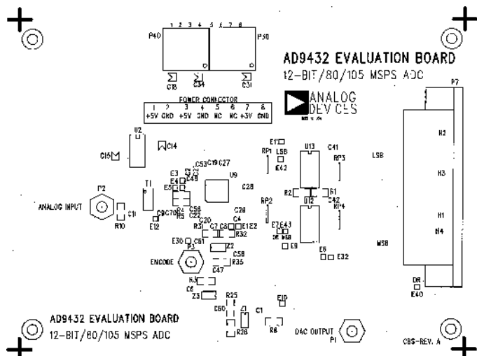
Figure 34. Top Silkscreen
