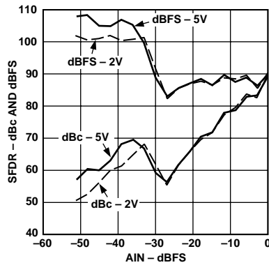
Figure 9. Single Tone SFDR ( f_{IN} = 1.5 MHz, V_{CM} = 2.5 V)
