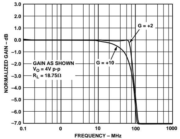
Figure 20. Large Signal Frequency Response; V_O = 4 V p-p
