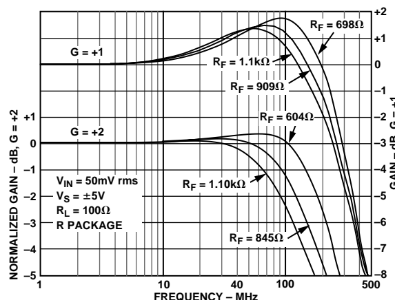
Figure 33. R_{FEEDBACK} vs. Frequency Response, G = +1/+2
