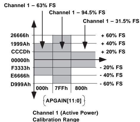
Figure 31 – Active Power Calculation Output Range
