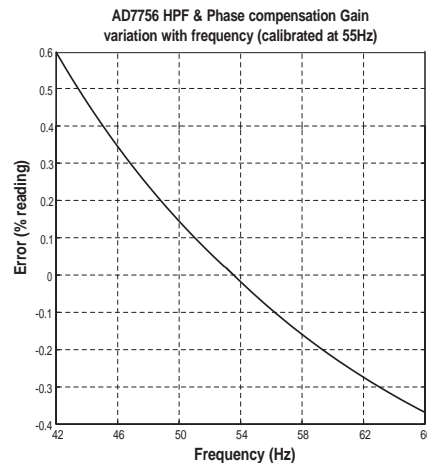
Figure 27c – Gain response of HPF & Phase Compensation (deviation of Gain as % of Gain at 54Hz)
