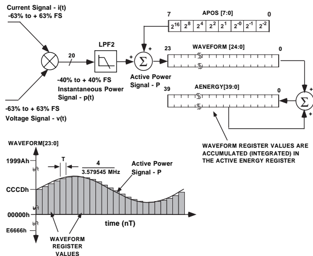
Figure 32 – AD7756 Energy Calculation
