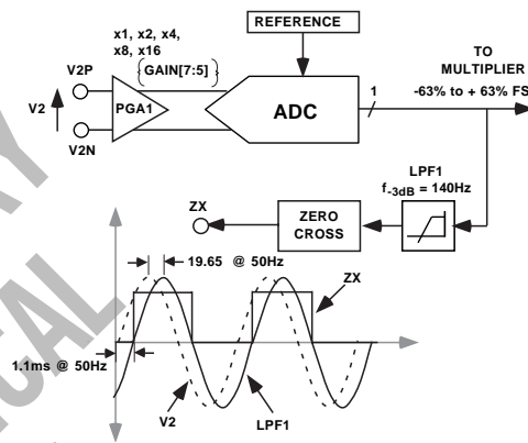
Figure 12– Zero cross detection on Channel 2
