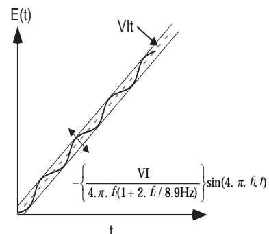
Figure 35 – Output frequency ripple
