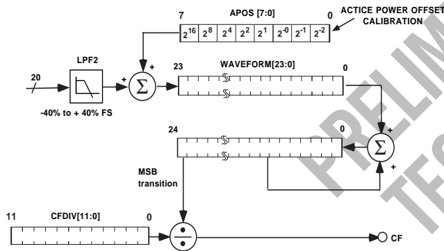
Figure 34– AD7756 Energy to Frequency Conversion
