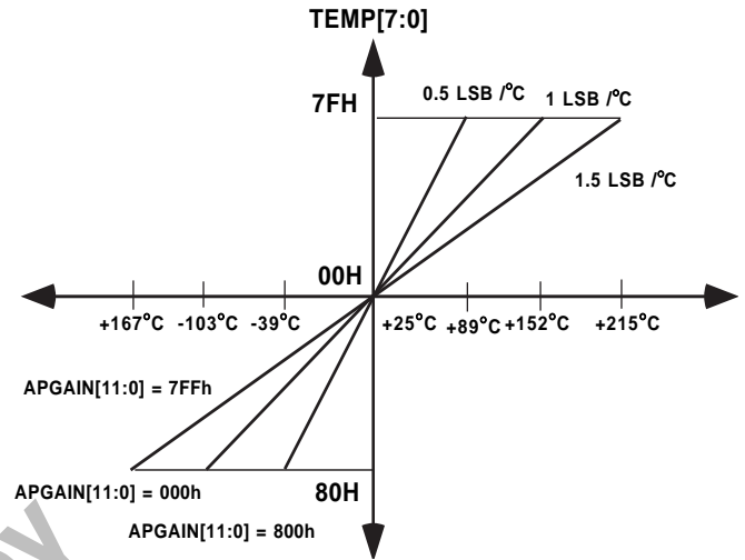
Figure 17– Temperature Register
