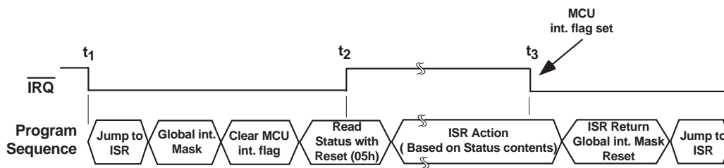
Figure 15– AD7756 interrupt management
