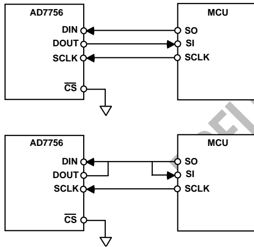
Figure 43 – Minimizing the Serial Interface
