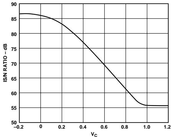
Figure 14. ISNR vs. Control Voltage—Low Ripple Mode
