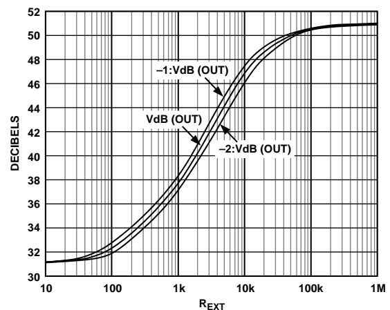
Figure 3. Gain vs. R_{\text{EXT}} , Showing Worst-Case Limits Assuming Internal Resistors Have a Maximum Tolerance of 20%
