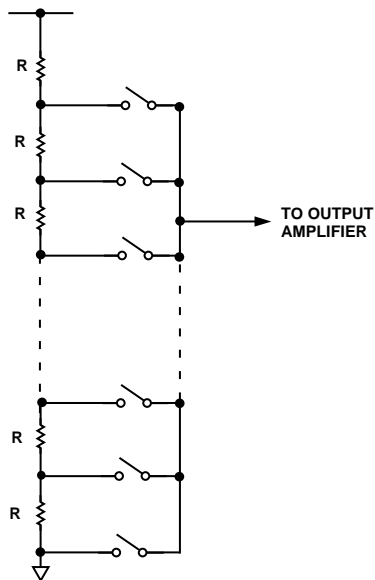
Figure 21. Resistor String
