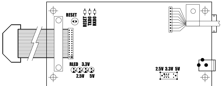
Figure 1. Jumpers
