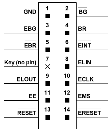
Figure 2a. Target board emulation header
