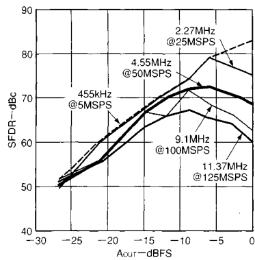
図27 . 1波のSFDRとA OUT @f OUT = f CLOCK /11
