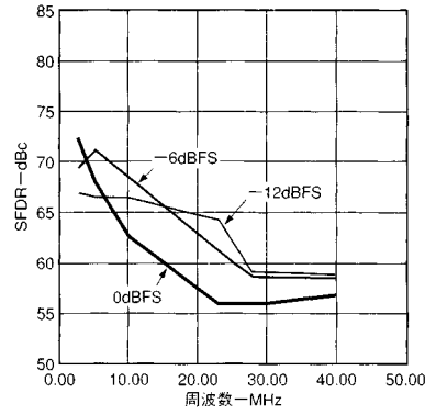
図25 . SFDRとf OUT @100MSPS
