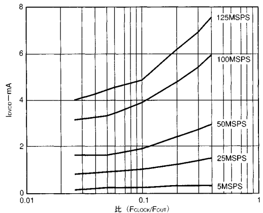
図49. I_{DVDD} と比率@DVDD = 3 V
