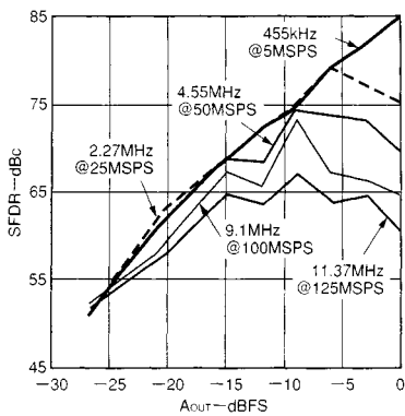
図9 . 1波のSFDRとA OUT @f OUT = f CLOCK /11
