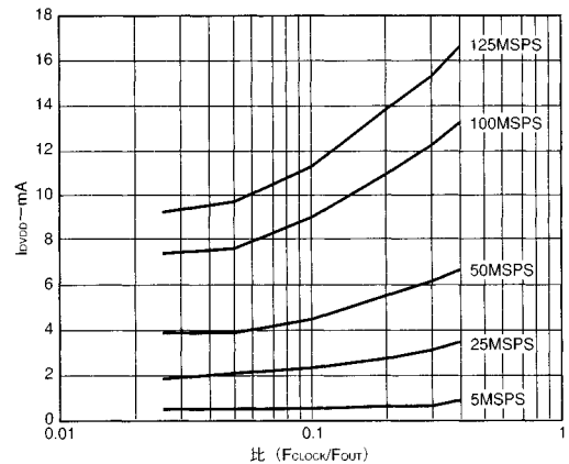
図48. I_{DVDD} と比率@DVDD = 5 V
