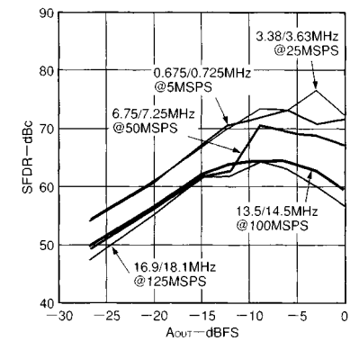
図29 . 2波のSFDRとA OUT @f OUT = f CLOCK /7
