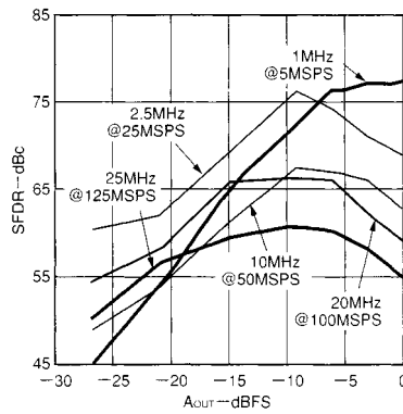
図10 . 1波のSFDRとA OUT @f OUT = f CLOCK /5
