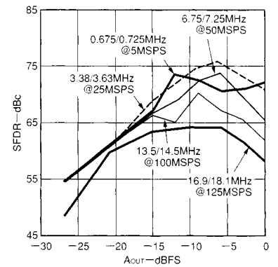
図11 . 2波のSFDRとA OUT @f OUT = f CLOCK /7
