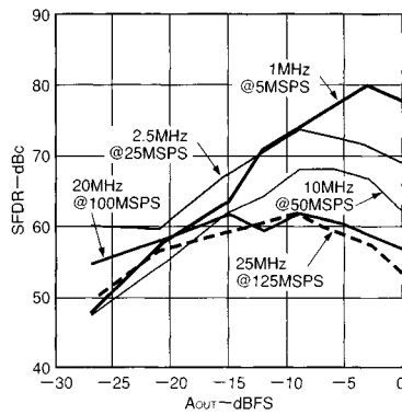
図28 . 1波のSFDRとA OUT @f OUT = f CLOCK /5
