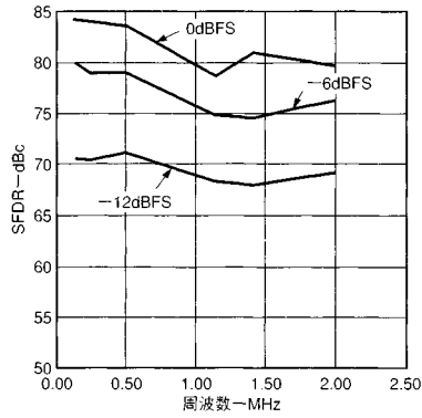
図22 . SFDRとf OUT @5MSPS
