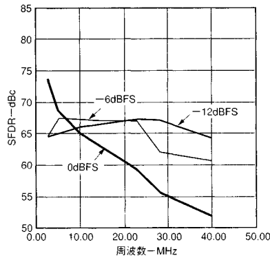
図7 . SFDRとf OUT @100MSPS
