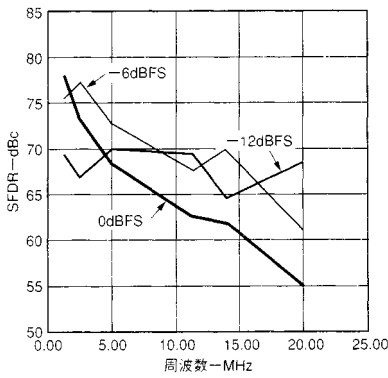
図6 . SFDRとf OUT @50MSPS
