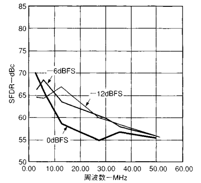
図26 . SFDRとf OUT @125MSPS
