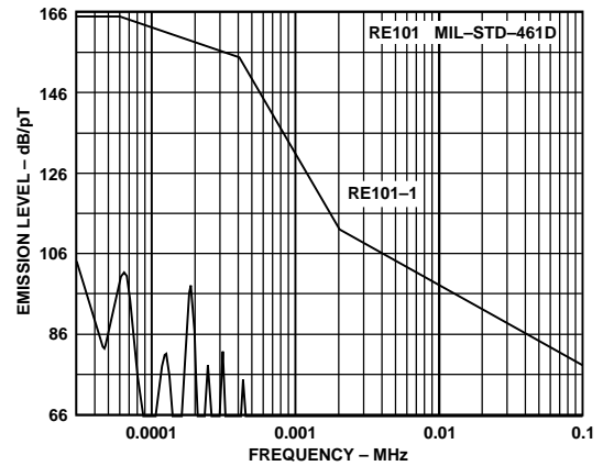
Figure 15. Radiated Emissions, MIL-STD-461D, RE101, 100 W Load
