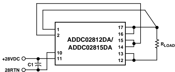
Figure 28. Typical Power Connections and External Parts for Converter
